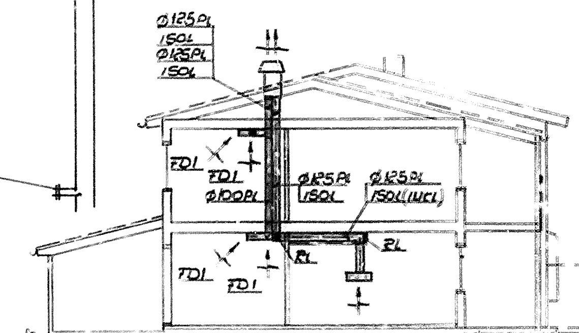
SECTION 1:100
